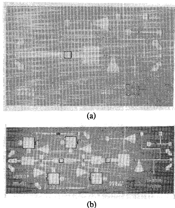
Fig. 1. The photograph of the monolithic 94 GHz (a) Schottky diode detector, and (b) preamplified detector.
